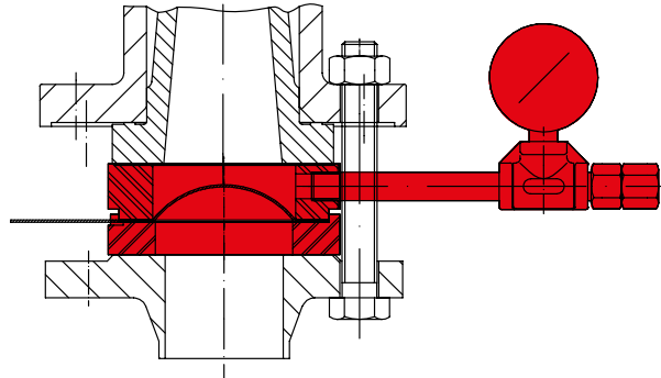
Rupture disc
