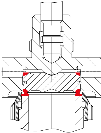
Nozzle SA479Gr.316Ti / Stellite No. 21 Disc SA479Gr.316Ti / Stellite No. 6
