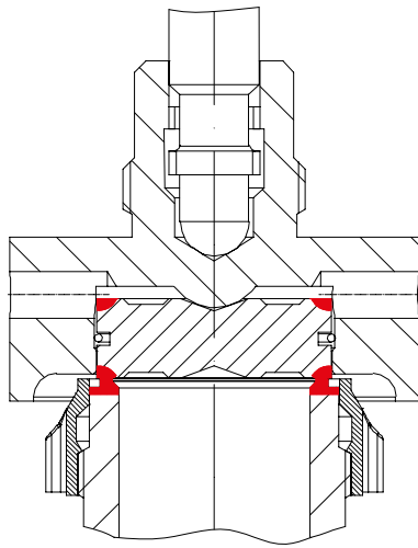
Nozzle SA479Gr.316Ti / Stellit No. 21 Kegel-Scheibe SA479Gr.316Ti / Stellit No. 6
