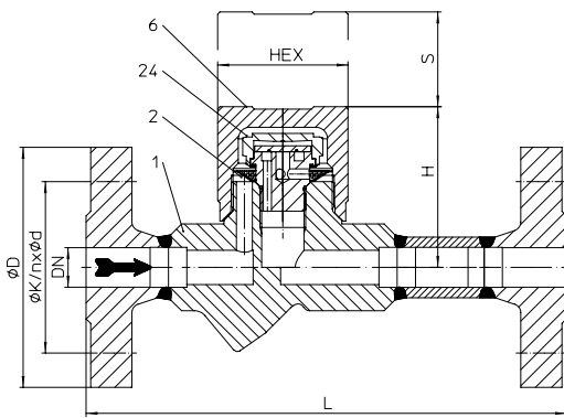
Fig. 640....1 with flanges
